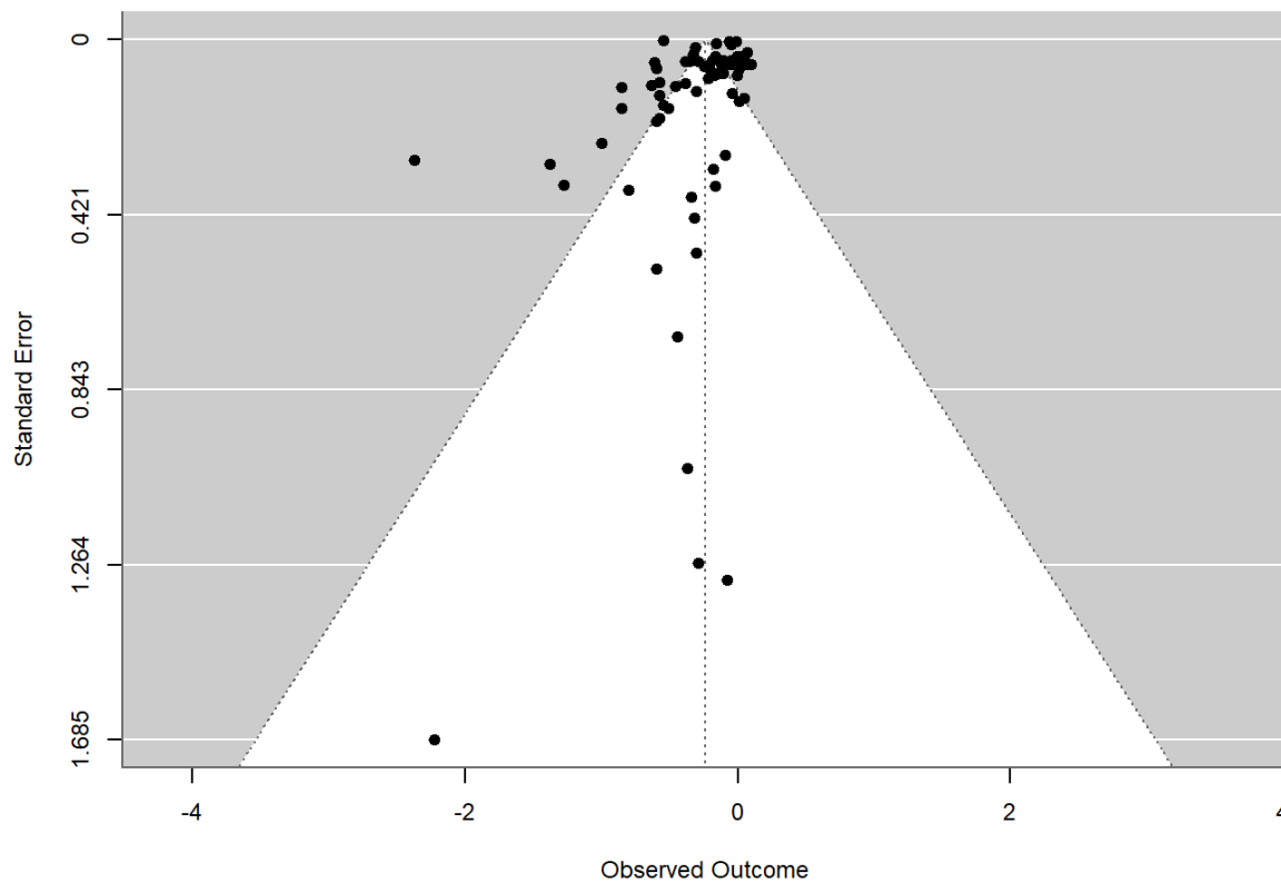
Figure 3 Funnel plot
